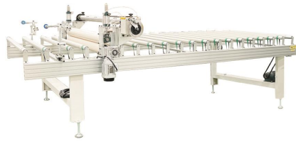
TBF 修长边+贴保护膜装置+输送排 TBF Long side trimming & protective film device & conveyor
