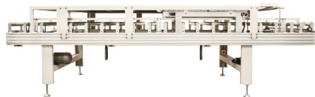
TSS-B 片材输送排 (保温烘道) TSS-B Sheet table conveyor with oven
